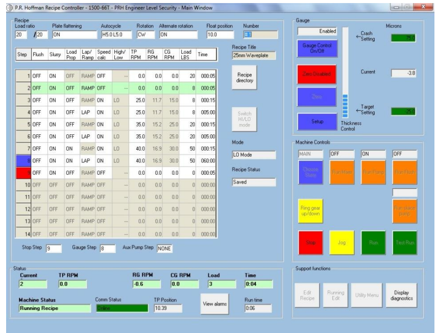
Servo RS™ Main Recipe Screen
